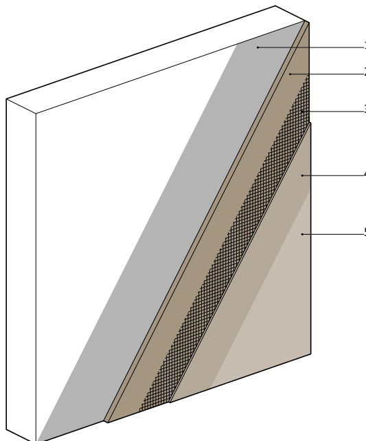
General scheme of a typical clay plaster build-up
