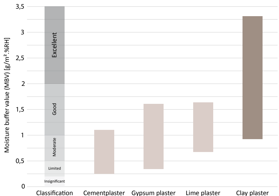
Moisture buffer value of clay plaster [4]
